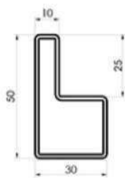
50×30×25 Step Beam Thickness: 1.2/1.5mm
