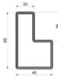
60×40×28 Step Beam Thickness: 1.2/1.5/2.0mm
