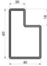
60×40×18 Step Beam Thickness: 1.2/1.5/2.0mm
