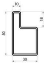
50×30×18 Step Beam Thickness: 1.2/1.5mm
